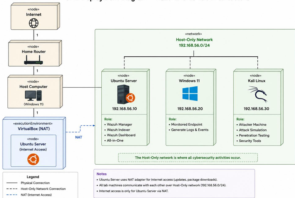
UML Deployment Diagram – Wazuh Home Lab Architecture
